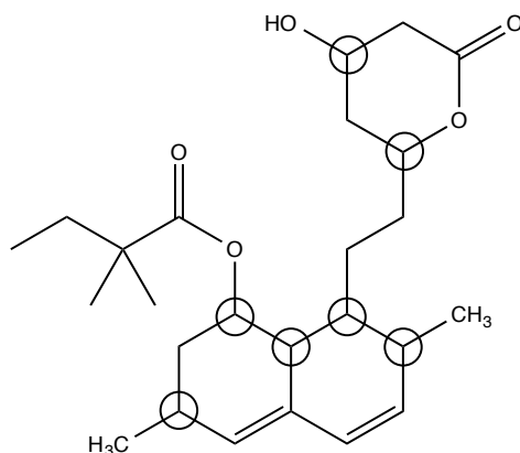
simvastatin
