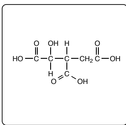
isocitric acid
