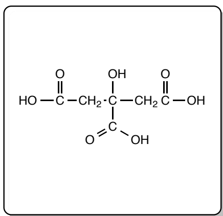
citric acid
