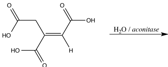
aconitic acid
