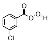
m-chloroperoxybenzoic acid (m-CPBA)
