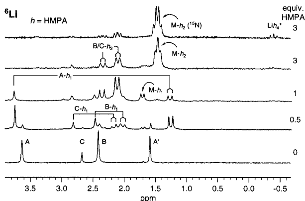
Figure 13. {}^6\text{Li} NMR spectra of \sim 0.16 M {}^6\text{Li} -labeled 1 in 3:2:1 THF/Me 2 O/Et 2 O at -135 °C. The top spectrum used {}^6\text{Li}/{}^{15}\text{N} double-labeled material and also contained TMEDA ( h = \text{HMPA} , M = \text{monomer} ).
