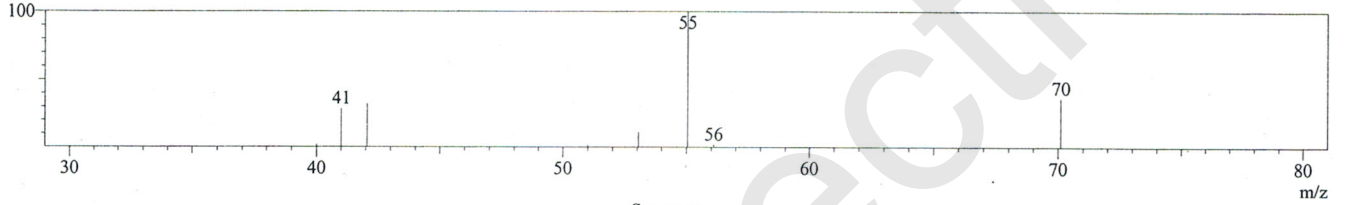
Peak#:2 R.Time:2.4(Scan#:74) MassPeaks:18
