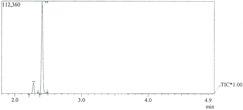
Peak#:1 R.Time:2.3(Scan#:59) MassPeaks:8
