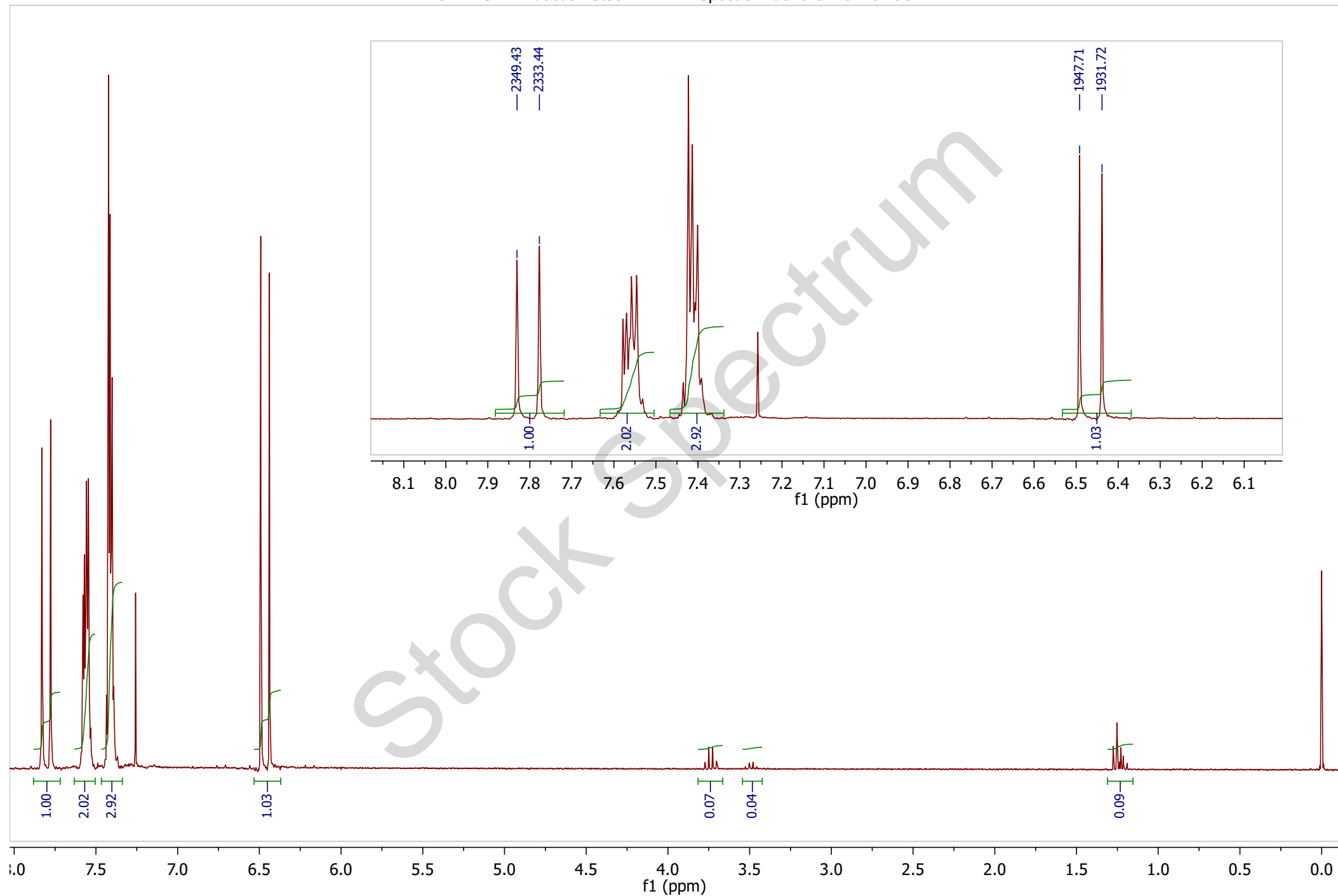
CHEM 344 Extraction Stock 1H-NMR Spectrum trans-Cinnamic Acid
