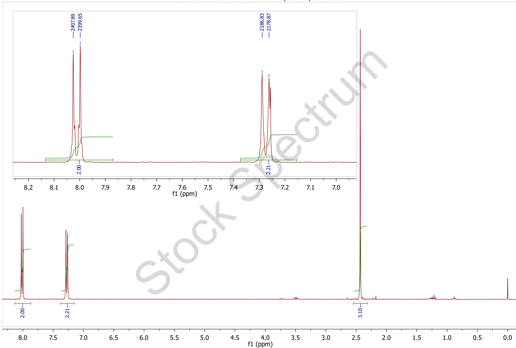
CHEM 344 Extraction Stock 1H-NMR Spectrum p-toluic acid
