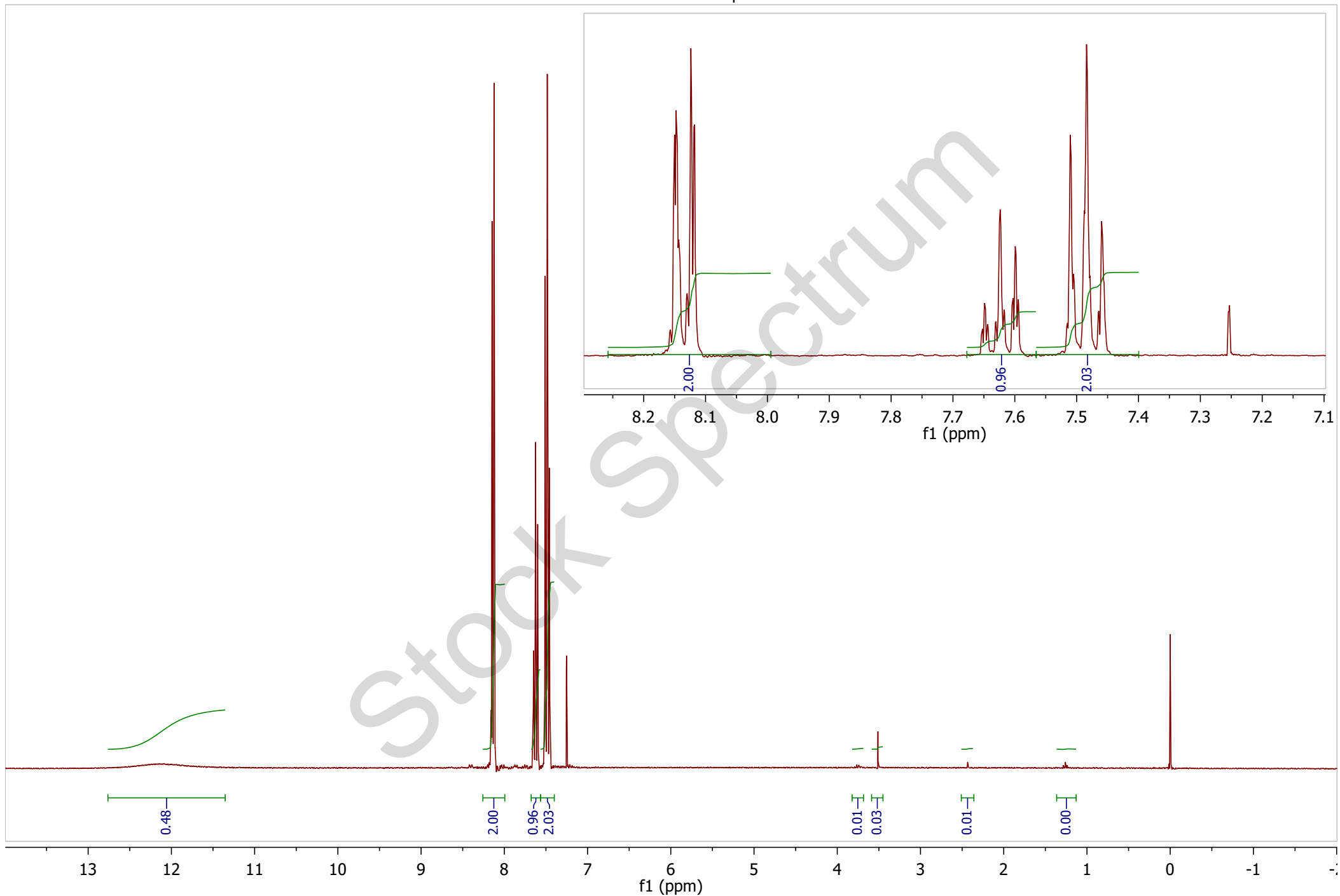
CHEM 344 Extraction Stock 1H-NMR Spectrum benzoic acid
