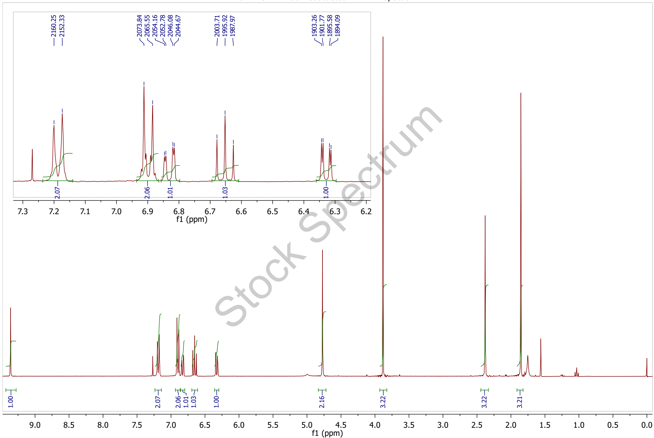
CHEM 344 Amide Product Stock 1H-NMR Spectrum
