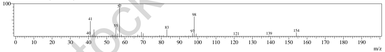
Peak#3 R. Time:4.1(Scan#:135) MassPeaks:55
