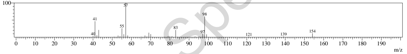
Peak#:2 R.Time:4.1(Scan#:135) MassPeaks:52
