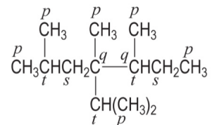
4-isopropyl-2,4,5-trimethylheptane
