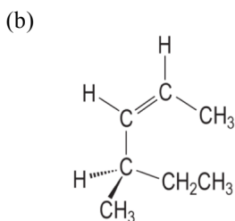
(2Z,4R)-4-methyl-2-hexene
