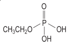
monoethyl phosphate
