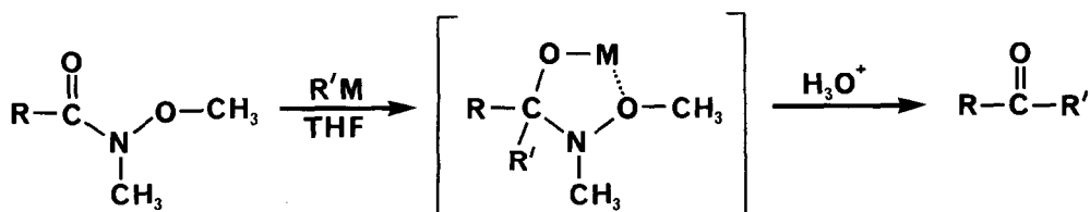
Scheme I
