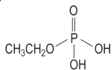
monoethyl phosphate
