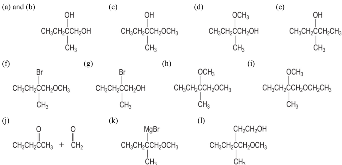
2-ethyl-2-methyloxirane
