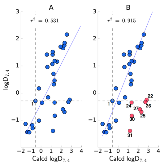
Figure 3. Comparison between experimental and calculated \log D_{7.4} values; (A) the linear regression for the entire data set; (B) the linear regression when major outliers (i.e., discrepancy >1 log unit, shown in red) are excluded.
